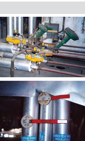
Pictured above: The function of the boiler drain and vent valves is to drain the boiler for maintenance outages. The valves are always closed when the boiler is in operation and must remain absolutely leak free while the plant is online – to ensure plant efficiency.
