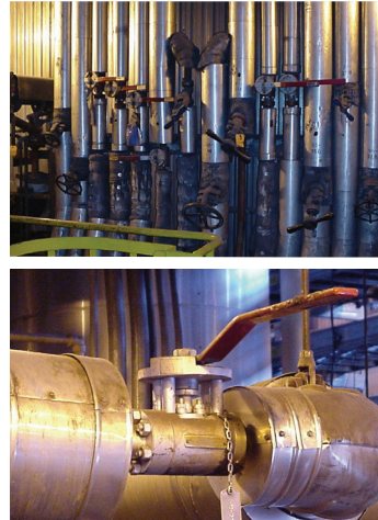
Pictured above: Main steam hot and cold reheat drain and vent valves. Steam is returned to the turbine in the hot reheat line at 1000°F (538°C), 600 psi (41 bar). The drain valves are used to heat the steam lines during start-up and discharge into condenser.
